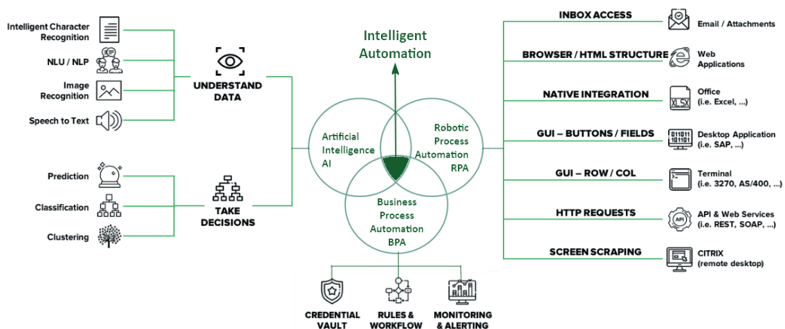
Figure 2. Intelligent Automation Components (modified from Reply, 2022)
