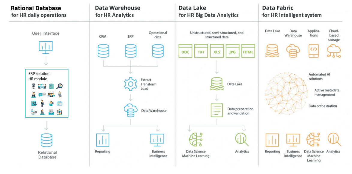
Figure 1. Comparison of different types of databases for HRM systems (modified from Kyslyi, 2022).
